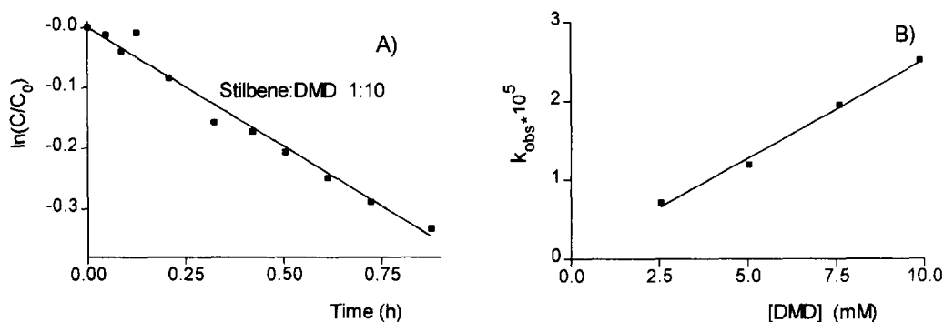
Figure 2. Kinetics of the DMD promoted epoxidation of cis -stilbene in \text{CHCl}_3 at 2 °C. a) Plot of \ln([cis\text{-stilbene}]/[cis\text{-stilbene}]_0) vs. time for the reaction with 10 fold excess of DMD, and b) plot of k_{obs} vs. [DMD] for the pseudo first order kinetics with different DMD excesses.
