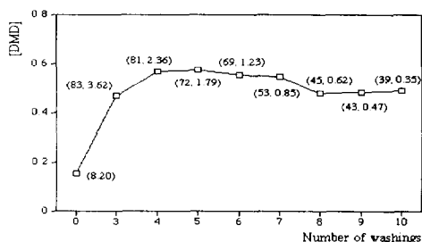
Figure 1. DMD Concentration obtained after successive washings of a \text{CH}_2\text{Cl}_2 extract (0.15 M) with 0.01 M phosphate buffer, pH 7. The percentage of DMD recovery and the corresponding molar acetone concentration remaining in the extract are given in parentheses.
